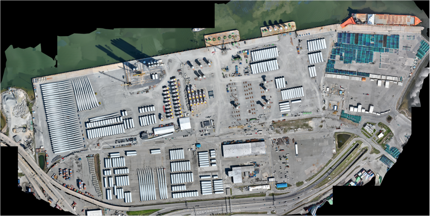
Figure 8: Portsmouth Marine Terminal – Staged WTG Components
