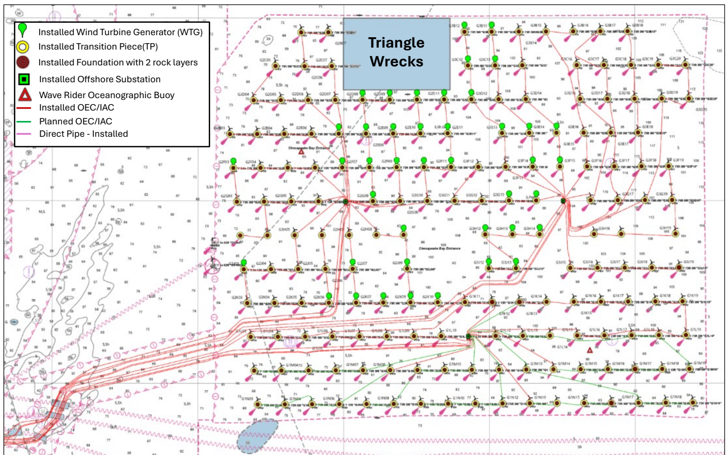
Figure 2: WTG and OSS Layout and Installation Status as of 30-SEP-2026
