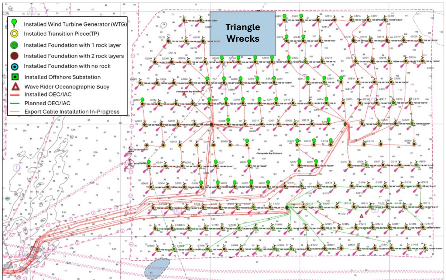
Figure 2: WTG and OSS Layout and Installation Status as of 31-AUG-2026
