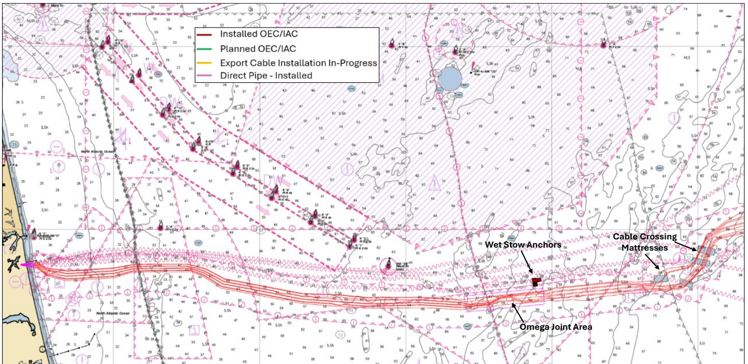
Figure 6: Positions for Omega Joint operations and cable crossings. Mariners should exercise caution when transiting in the vicinity of the Omega Joint Operations; vessels are extremely limited in maneuverability during cable jointing activity.
