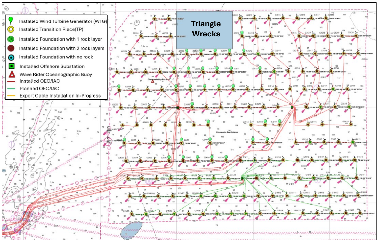
Figure 2: WTG and OSS Layout and Installation Status as of 31-JULY-2026
