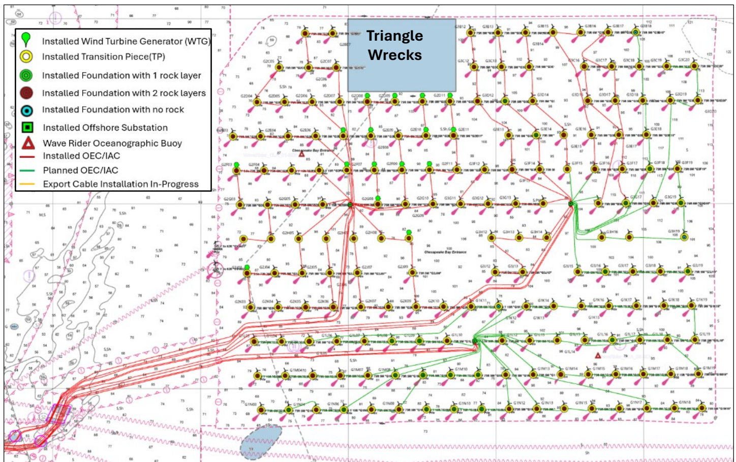
Figure 2: WTG and OSS Layout and Installation Status as of 31-MAY-2026
