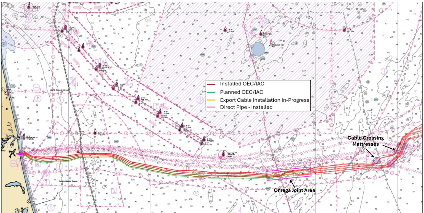
Figure 8: Positions for Omega Joint Operations and Cable Crossings are highlighted. Mariners should exercise caution when transiting in the vicinity of the Omega Joint Operations; vessels are extremely limited in maneuverability during cable jointing activity.
