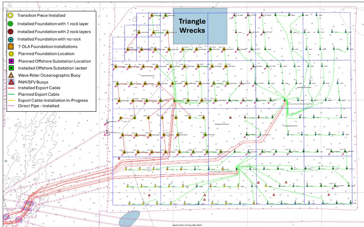
Figure 2: WTG and OSS Layout and Installation Status as of 30-AUG-2025
