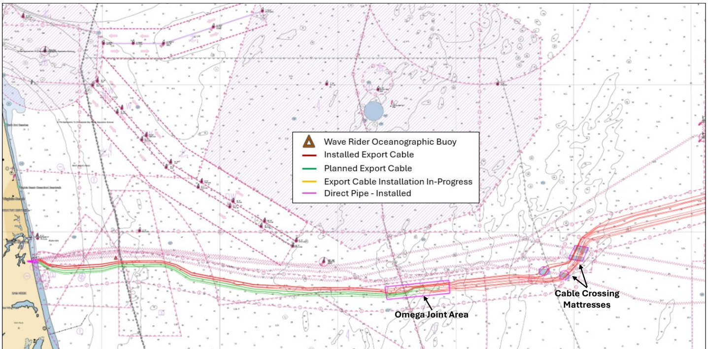
Figure 3: OEC Installation Status as of 30-AUG-2025; positions for Omega Joint Operations and Cable Crossings are highlighted. Mariners should exercise caution when transiting in the vicinity of the Omega Joint Operations; the vessel is extremely limited in maneuverability due to cable jointing activity.
