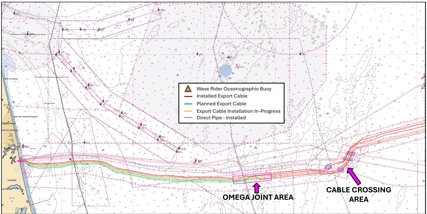
Figure 3: OEC Installation Status as of 30-JULY-2025; positions for Omega Joint Operations and Cable Crossings are highlighted. Mariners should exercise caution when transiting in the vicinity of the Omega Joint Operations; the vessel is extremely limited in maneuverability due to cable jointing activity.
