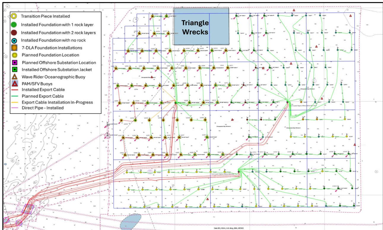
Figure 2: WTG and OSS Layout and Installation Status as of 30-JUL-2025
