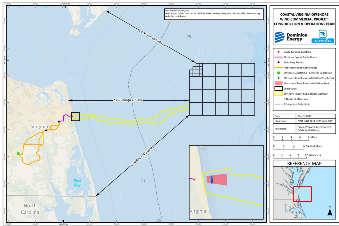
Figure 1. CVOW-C lease development area and export cable corridor.
